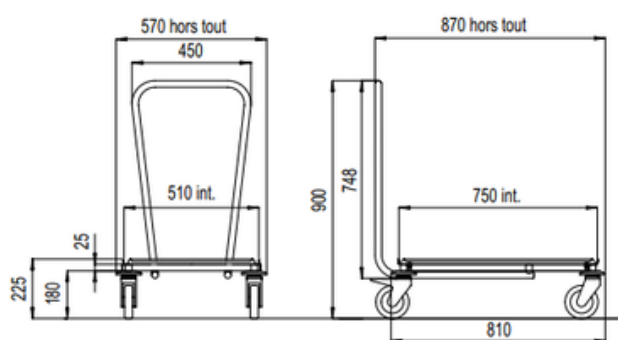
tray dollies
