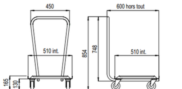
general purpose tray dollies
