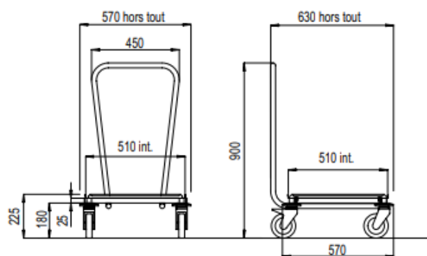
rack dollies with s/steel base
