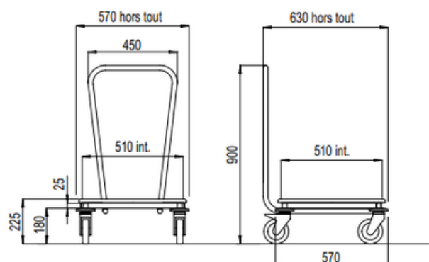
rack dollies with ABS base
